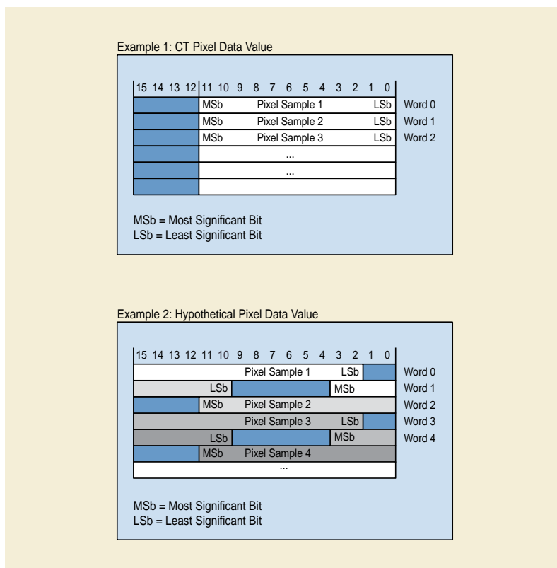
Figure D-4. Example Pixel Cells Packed into 16-bit Words (VR = OW)
