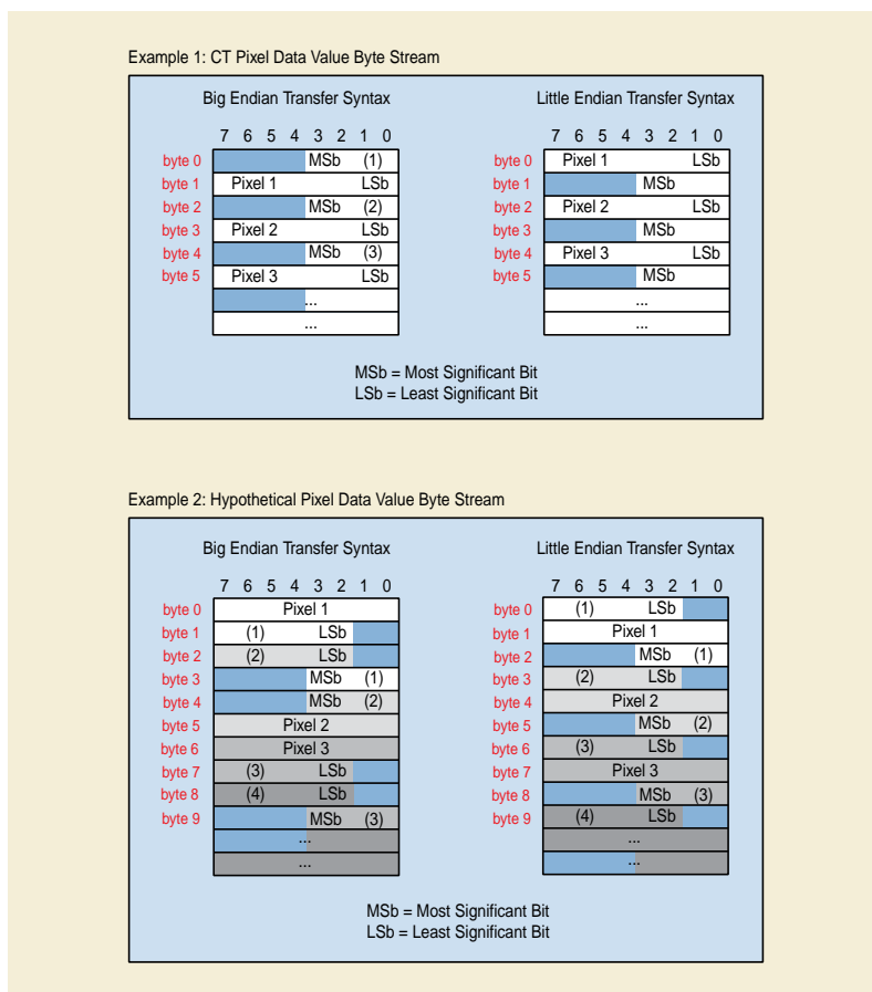
Figure D-6. Sample Pixel Data Byte Streams (VR = OW)
