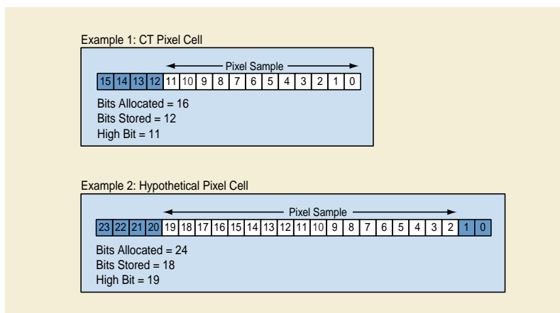
Figure D-3. Example Pixel Cells
